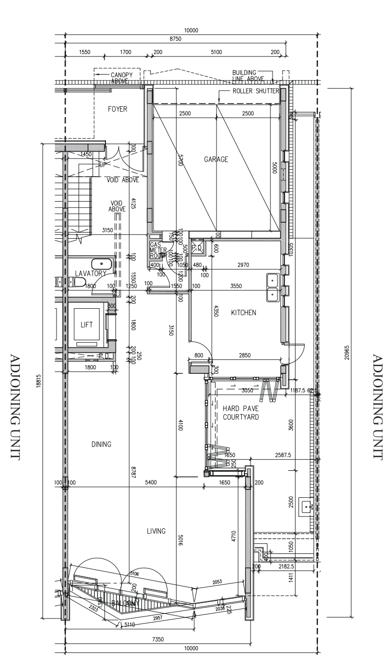
Unit A, No. 35 Blue Pool Road – 1/F to Roof Floor Plan
